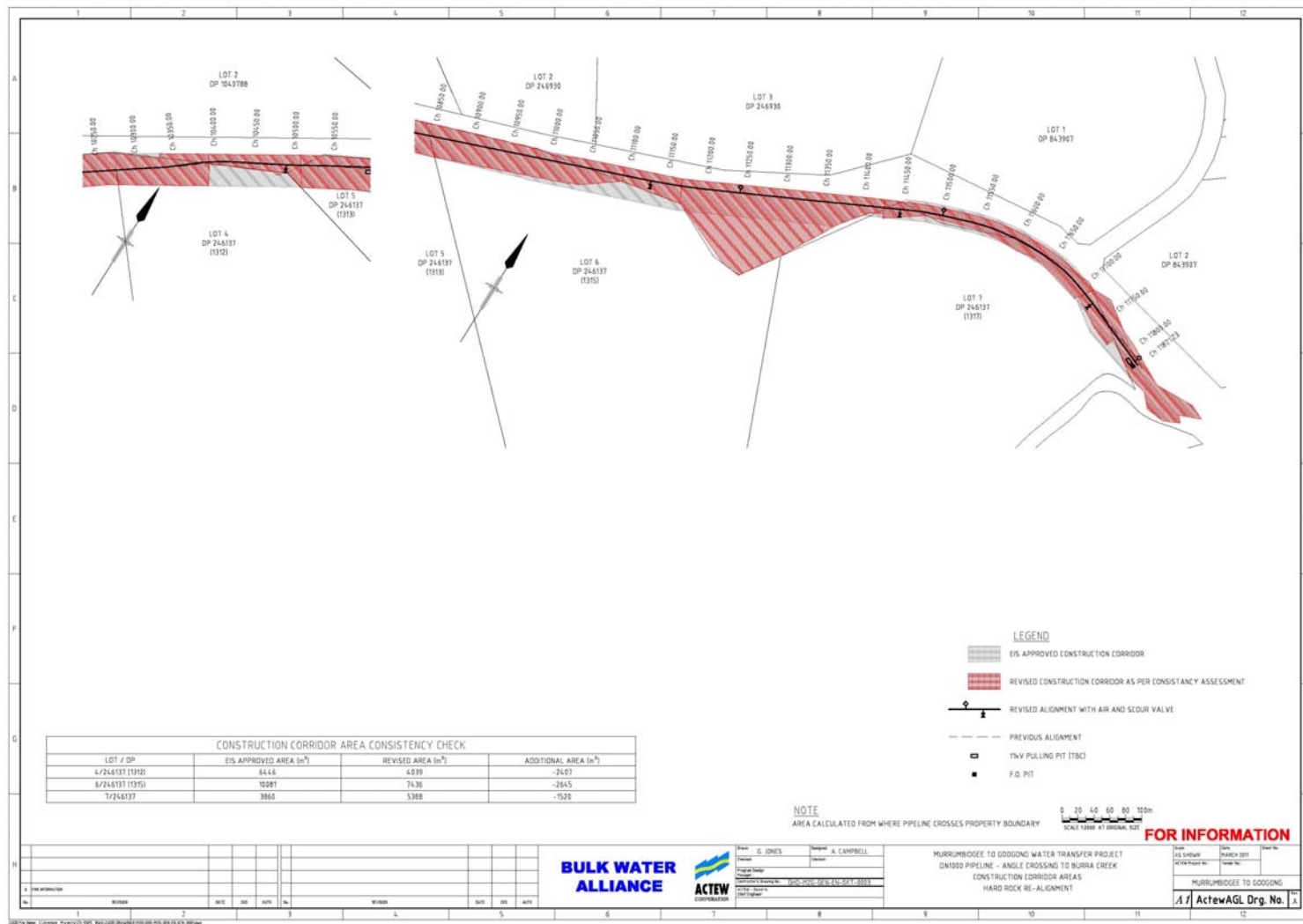
Figure 3 Approved Project Route and Proposed Design Alteration for properties 1313 and 1315
