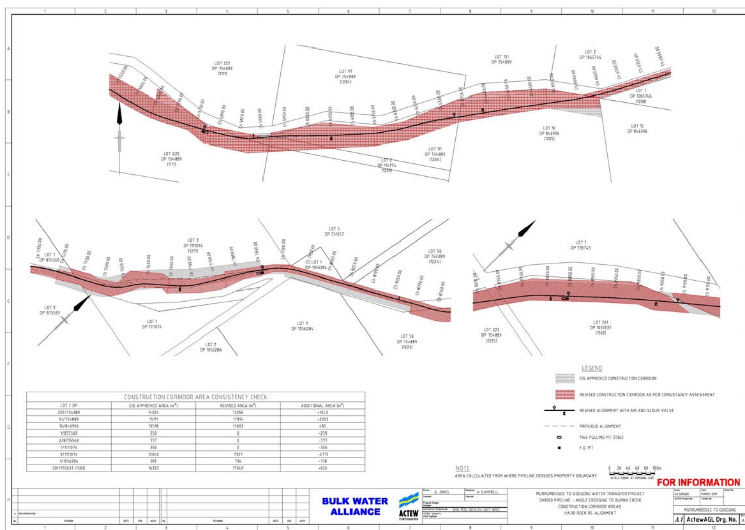
Figure 2: Approved Project Route and Proposed Design Alteration for properties 1111, 1217 and 1302
